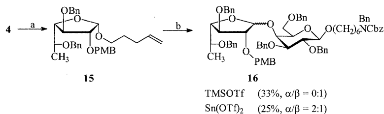
Scheme 4. Intermolecular glycosidic coupling: (a) PMBCl, NaH, DMF (91%); (b) 5 , NIS, Lewis catalyst, CH 2 Cl 2
