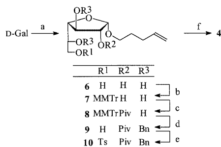
Scheme 2. Synthesis of \alpha -D-fucufuranoside 4 : (a) 4-penten-1-yl bromide, NaH, DMPU; Ac 2 O, Pyr; MeONa, MeOH (37%); (b) MMTrCl, DMAP, Pyr (75%); (c) PivCl, Pyr (77%); (d) BnBr, TBAI, NaH, CH 2 Cl 2 ; IR 120 (H + form) (85%); (e) TsCl, Et 3 N, DMAP, CH 2 Cl 2 (94%); (f) NaBH 4 , DMF; MeONa, MeOH (77%)
