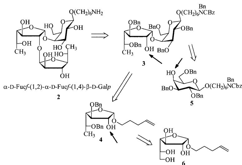
Scheme 1. Targeted mimic structures and retrosynthetic approach
