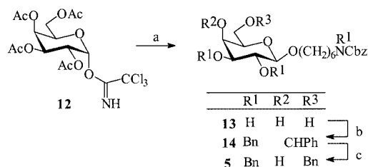
Scheme 3. Synthesis of \beta -D-galactopyranoside 5 : (a) HO(CH 2 ) 6 NHCbz ( 11 ), Sn(OTf) 2 , CH 2 Cl 2 ; MeONa, MeOH (87%); (b) PhCH(OMe) 2 , CSA, DMF; BnBr, NaH, DMF (54%); (c) NaBH 3 CN, TfOH, THF (73%)
