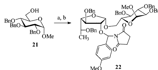
Scheme 6. Synthesis of \alpha -D-fucopyranoside 22 : (a) 15 , DDQ, CH 2 Cl 2 ; (b) NIS, CH 2 Cl 2 (21% for 2 steps)
