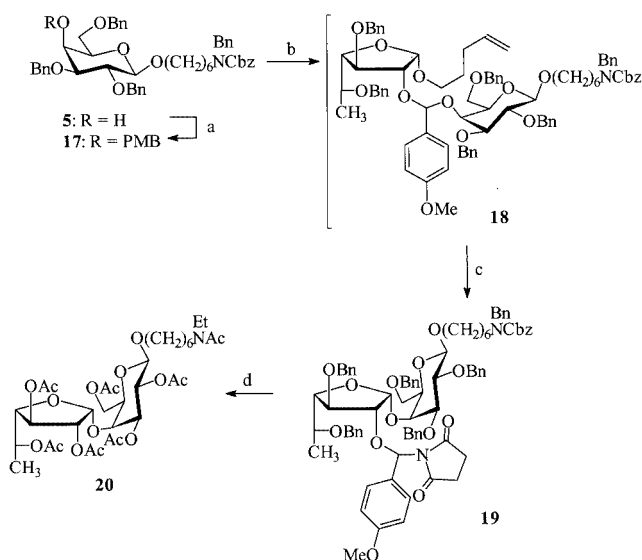
Scheme 5. Tethering and intramolecular aglycon transfer: (a) PMBCl, NaH, DMF (90%); (b) 4 , DDQ, CH 2 Cl 2 ; (c) NIS, CH 2 Cl 2 (34% for two steps); (d) H 2 (30 atm), Pd(OAc) 2 , Ac 2 O, Py (25%)
